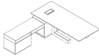
2100mm x 2075mm XE-W2109R2004- NBA4-ML/LM-L
