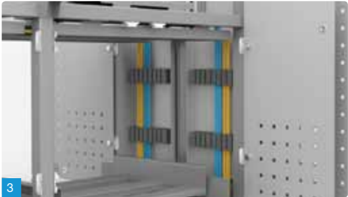
Vertical Cable Channel
