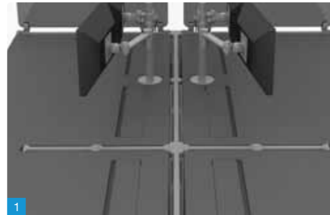
2mm gap between tabletop and panels
